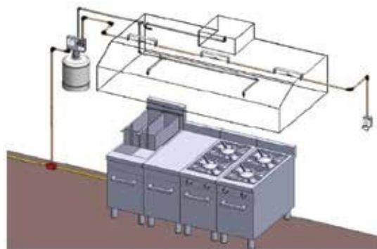
Cooking area and hood extinguishing system
